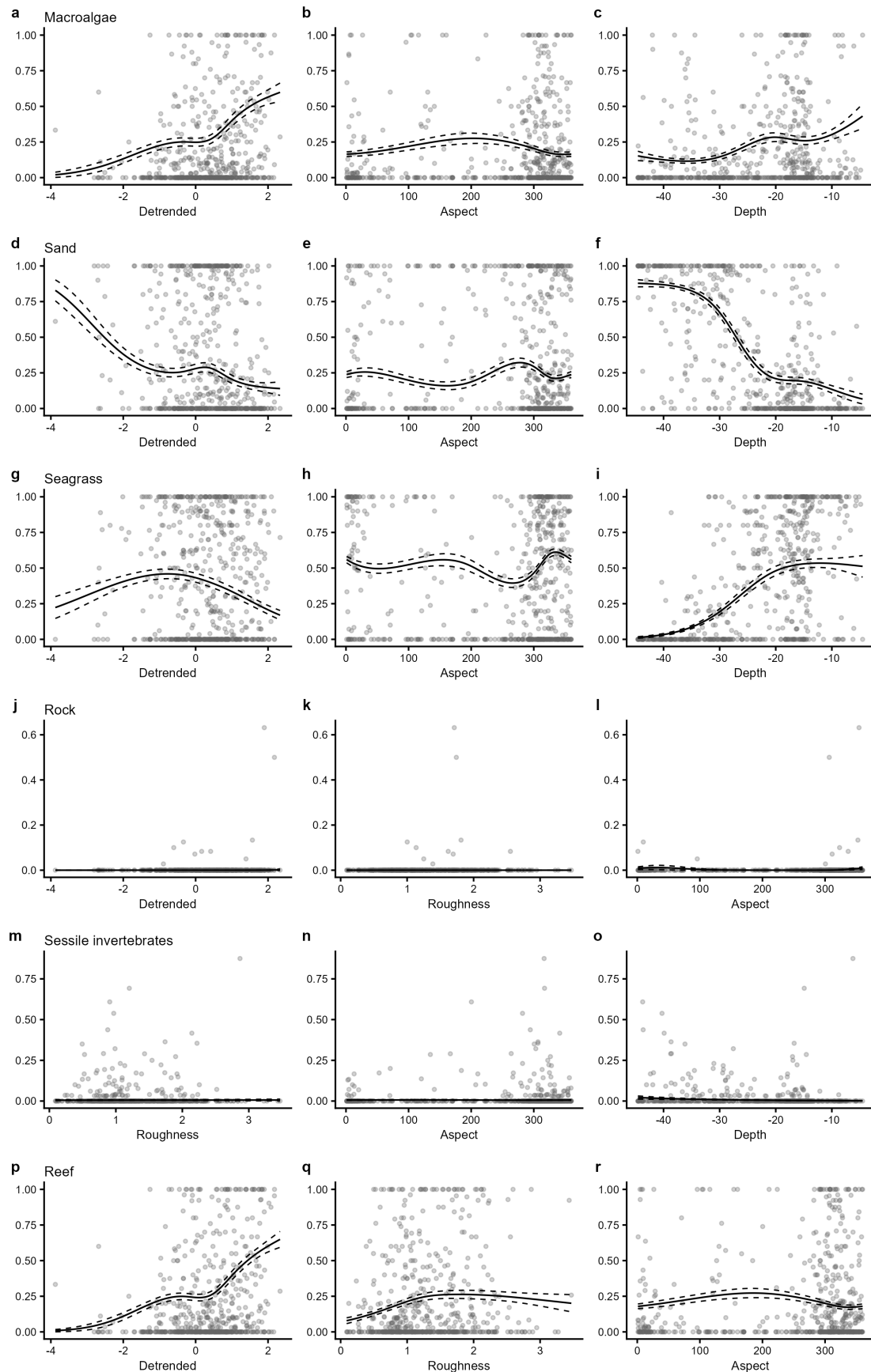
Figure C 1.2: Plots of the most parsimonious model found to predict the probability of occurrence of key habitat types. Individual panes display the predicted relationships between model covariates and the probability of occurrence of each habitat class. Solid lines represent predicted Generalized Additive Model (GAM) fits with other variables held constant at their mean value. Dashed lines represent upper and lower standard error bounds around the prediction, and points represent the observed data from all
